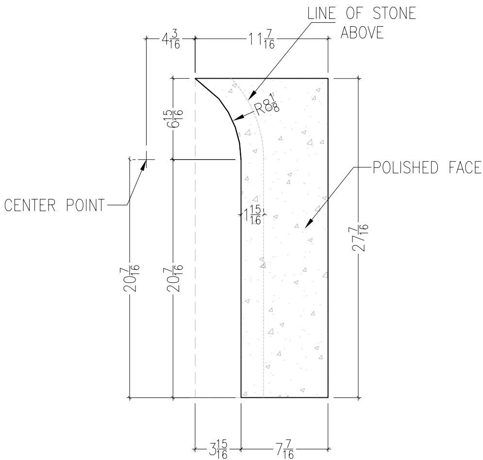
FRONT VIEW SCALE : 1 1/2" = 12"
