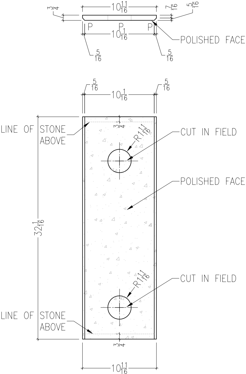
BOTTOM VIEW SCALE : 1 1/2" = 12"
