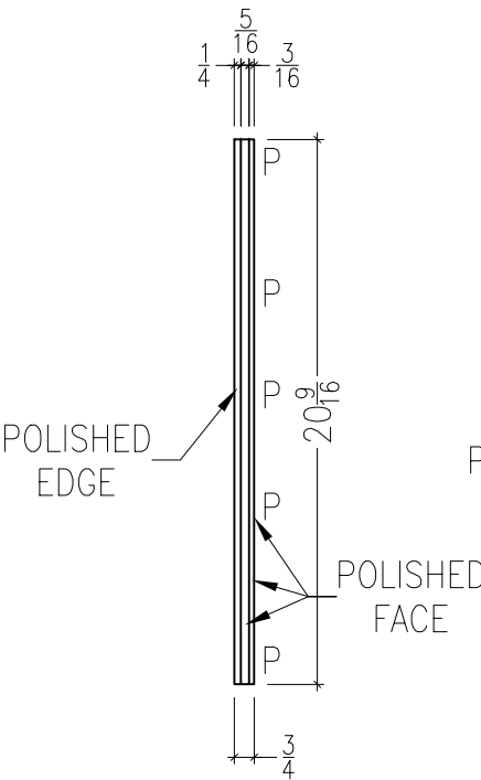
LEFT VIEW
