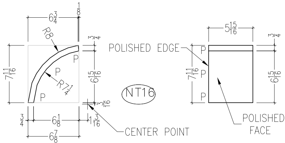
LEFT VIEW
