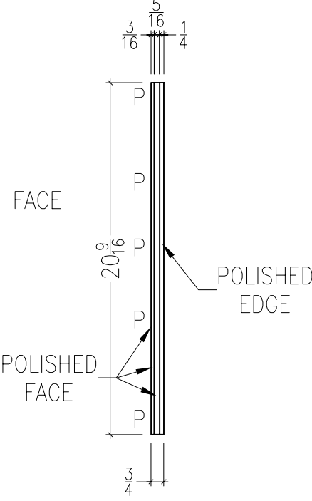
RIGHT VIEW
