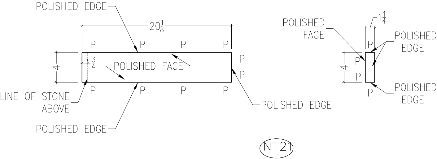
FRONT VIEW SCALE : 1 1/2" = 12"
