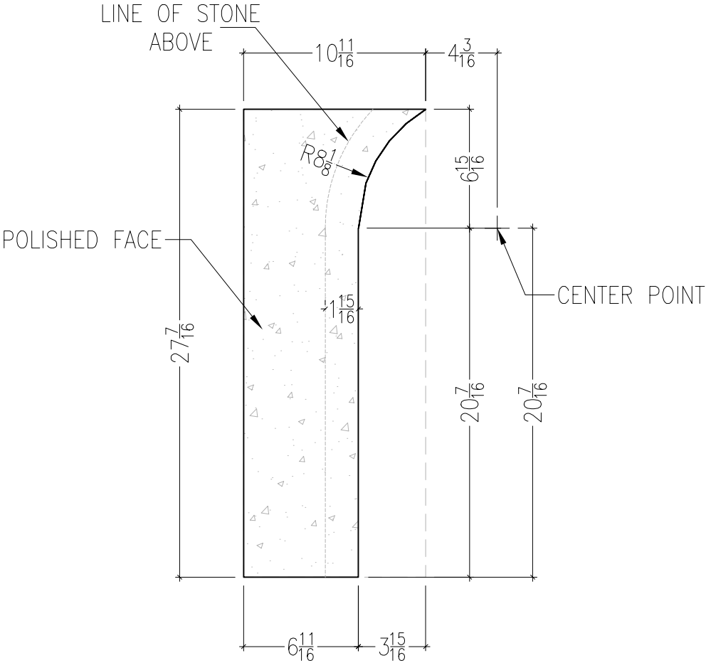
FRONT VIEW SCALE : 1 1/2" = 12"
