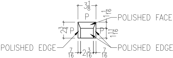
FRONT VIEW SCALE : 1 1/2" = 12"
