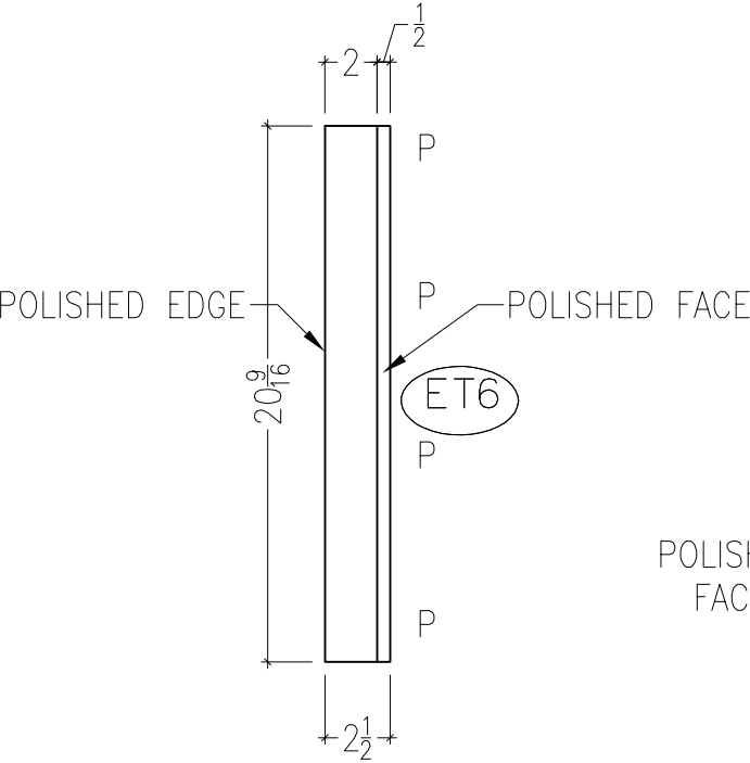
FRONT VIEW SCALE : 1 1/2" = 12"
