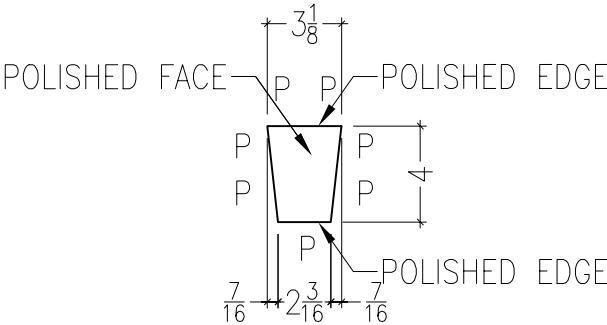
FRONT VIEW SCALE : 1 1/2" = 12"
