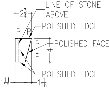
LEFT VIEW
