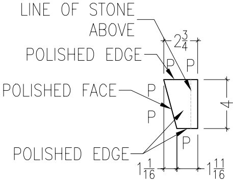
RIGHT VIEW
