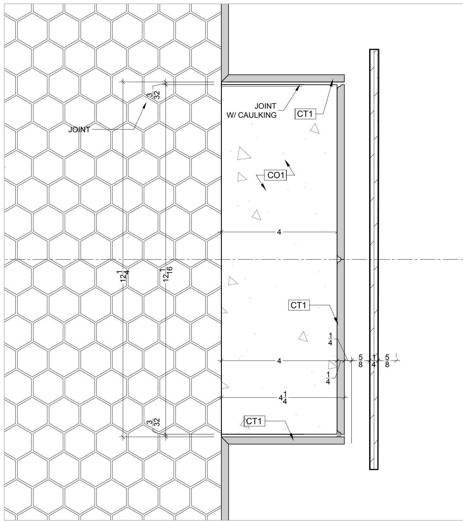
DETAIL @ NICHE Scale: 6"=1'-0"
