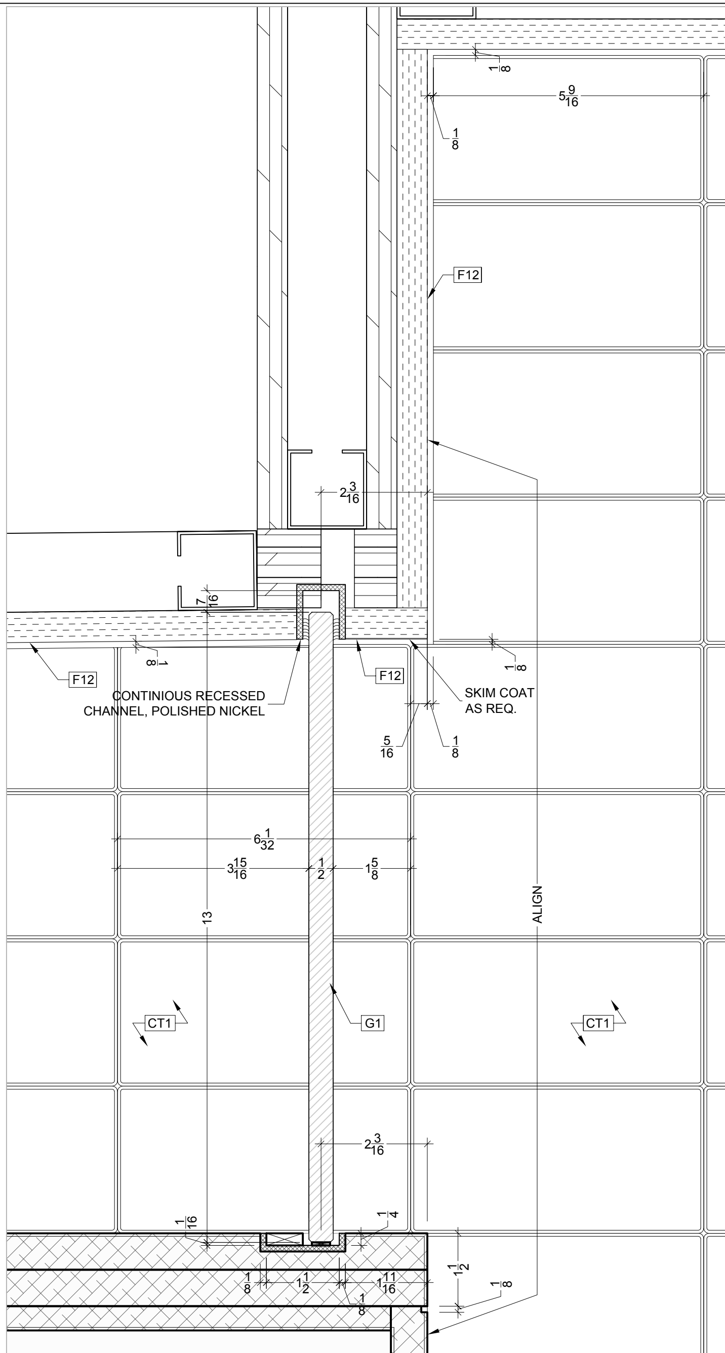
4 DETAILS @ GLASS PANEL Scale: 6"=1'-0"
