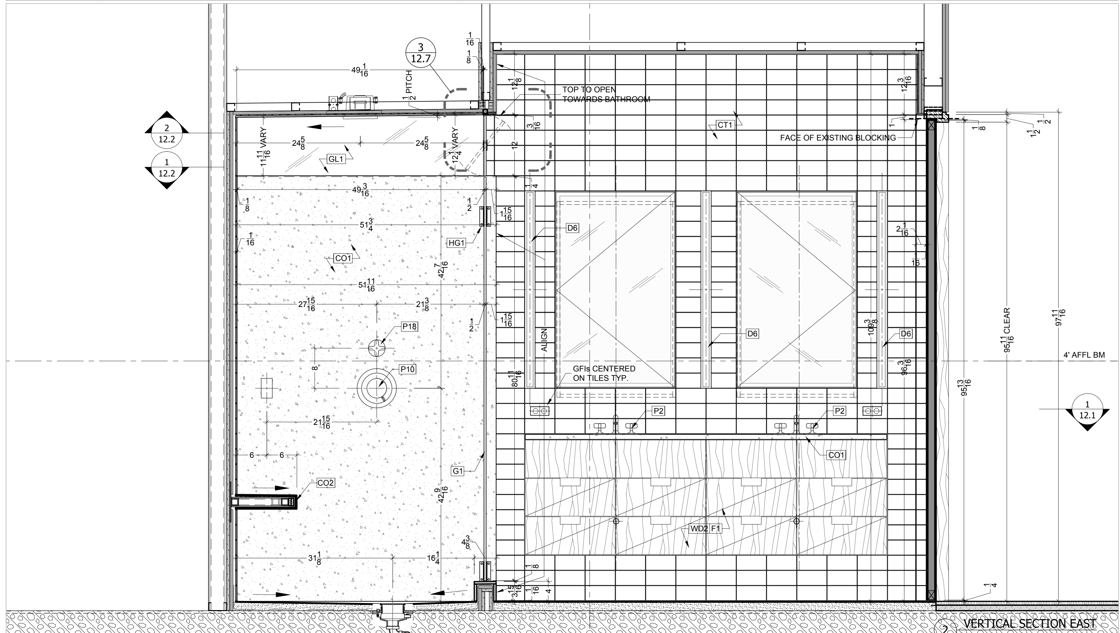
2 VERTICAL SECTION EAST Scale: 1/2"=1'-0"
